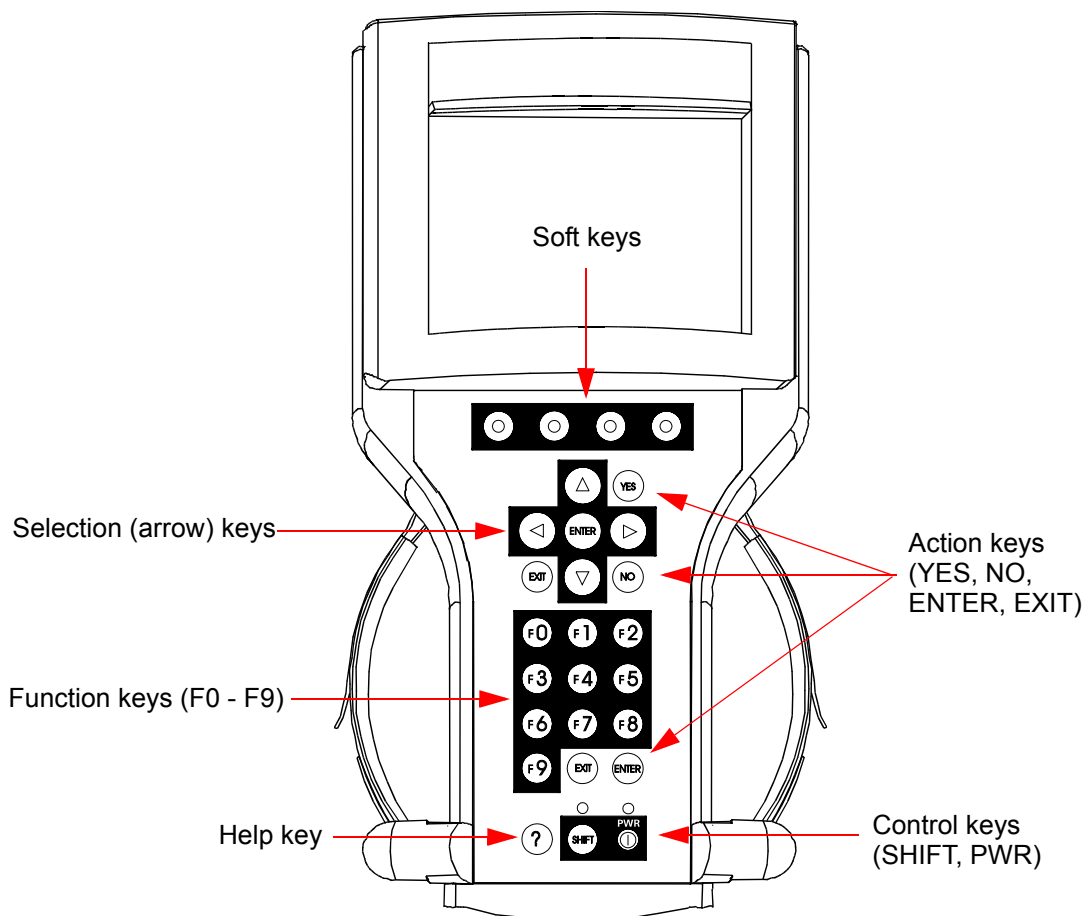
FIGURE 3-14. Tech 2 Keypad
